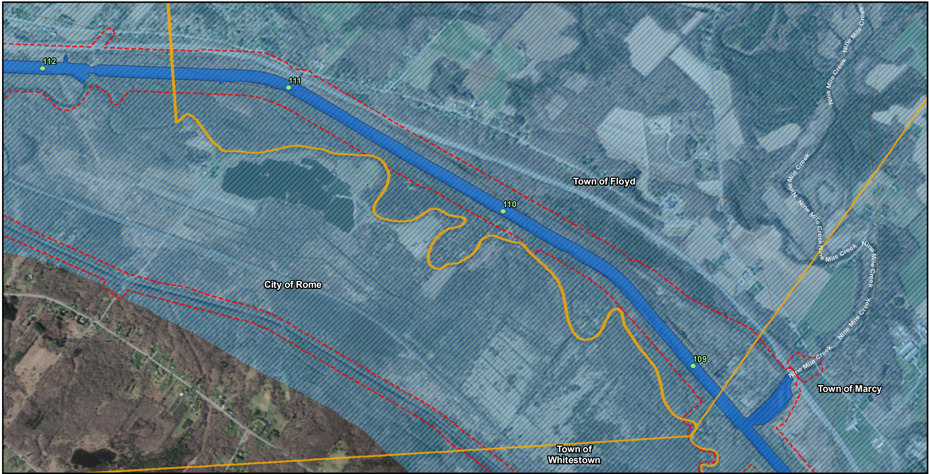
Figure 48F: Aquifers
